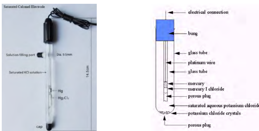
Fig 5.2.2: Calomel Electrode: a) commercial version, b) the anatomy of the electrode.
