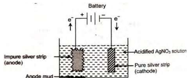
Fig: Electrolytic refining of silver
