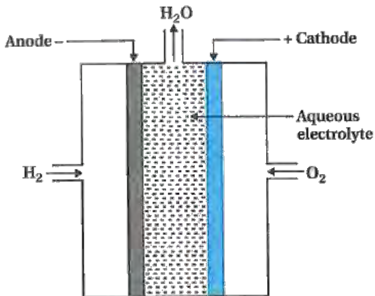
Fig 5.7.4: Hydrogen / Oxygen cell
