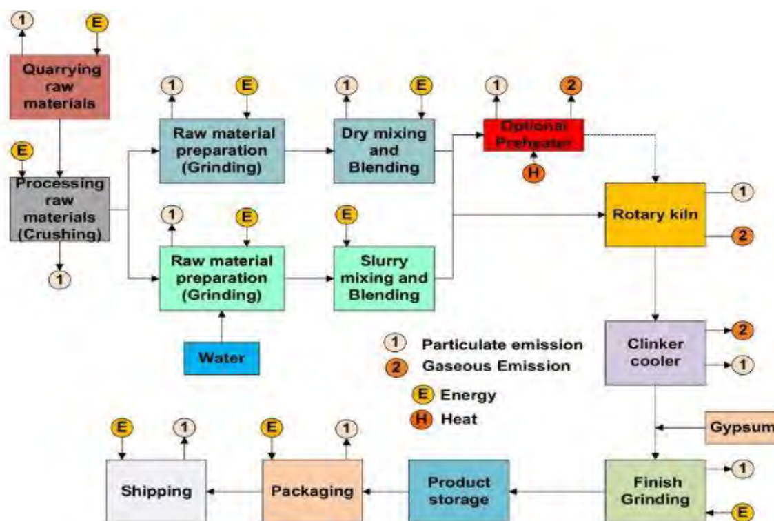
Fig: Sequential steps involved in production of cement
