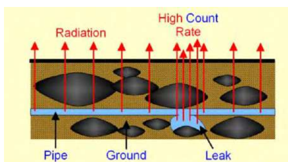
Fig: Use of radioisotope to detect leakage in pipeline
