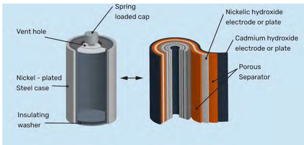
Fig 5.7.3: Ni-Cd Battery
