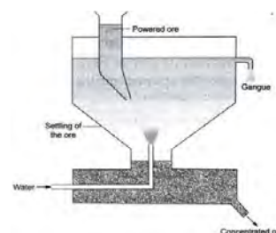
Fig: Gravity Separation
