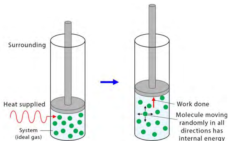
Figure: energy is absorbed by the system and does some work
