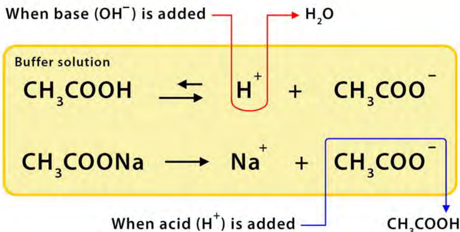
Figure: Mixture of weak acid ( \text{CH}_3\text{COOH} ) and its salt with strong base ( \text{CH}_3\text{COONa} ) which act as an acidic buffer
