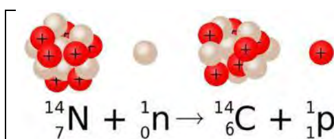
Fig: Formation of C-14
