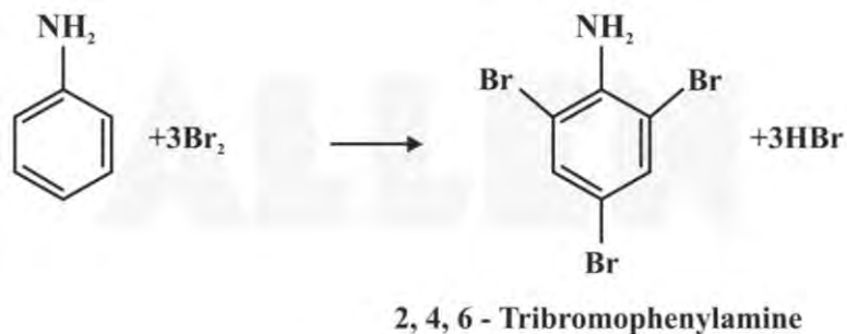
Bromine water test with aniline
