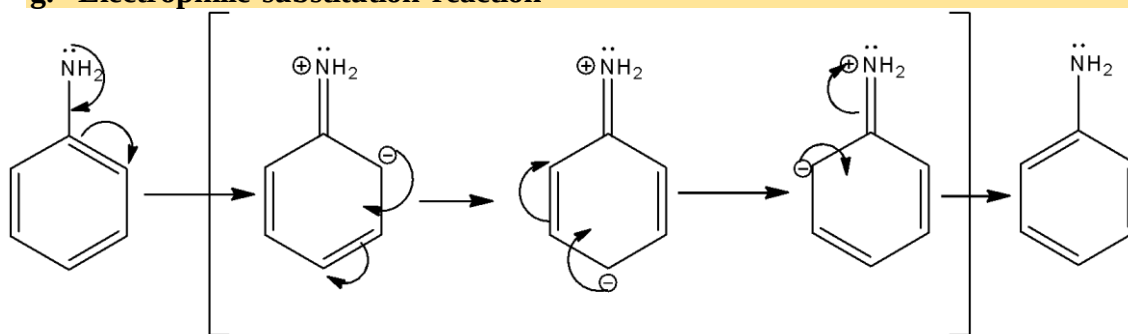
Resonance structures of Aniline
