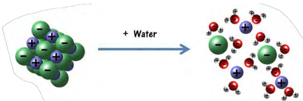
Figure: degree of ionization increases with the addition of water
