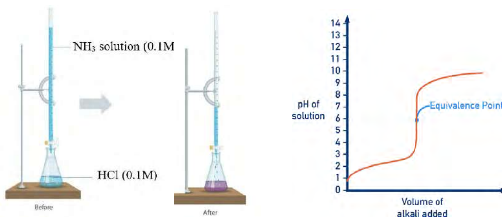
Figure: A graph of pH versus volume of alkali in the titration of strong acid and weak base
