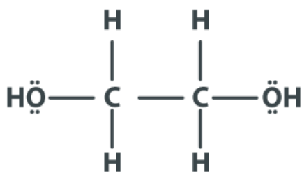
Ethylene Glycol (Ethan-1,2-diol)
