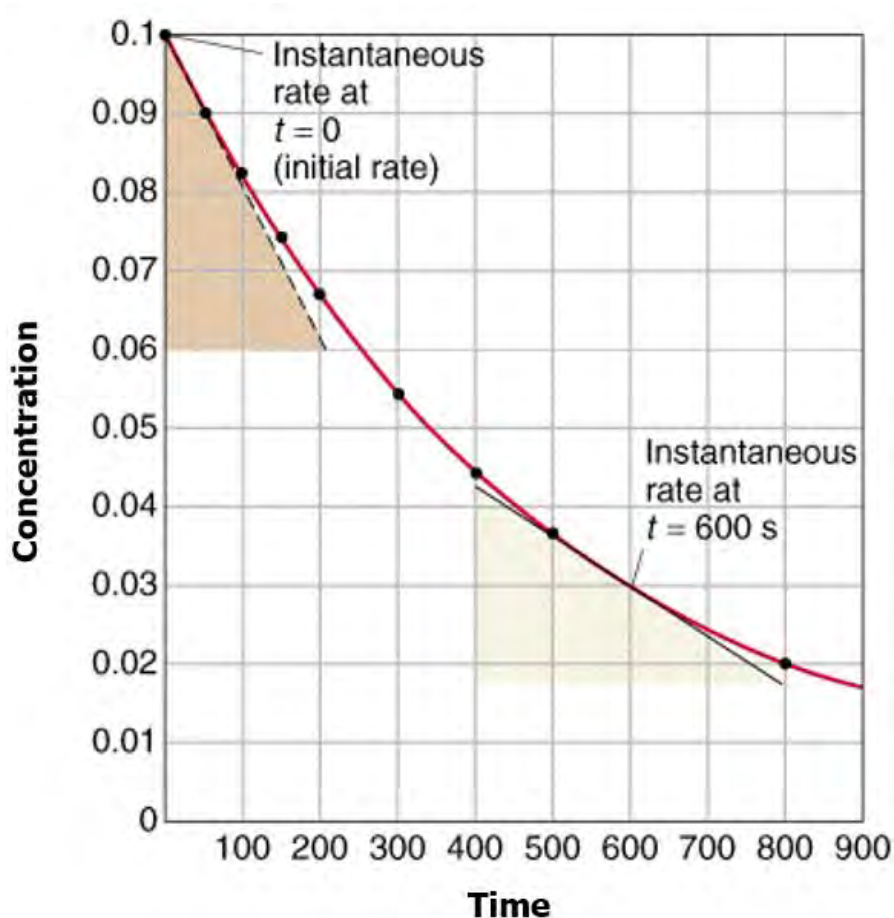
Figure: the tangent of the slope of the graph gives the instantaneous rate
