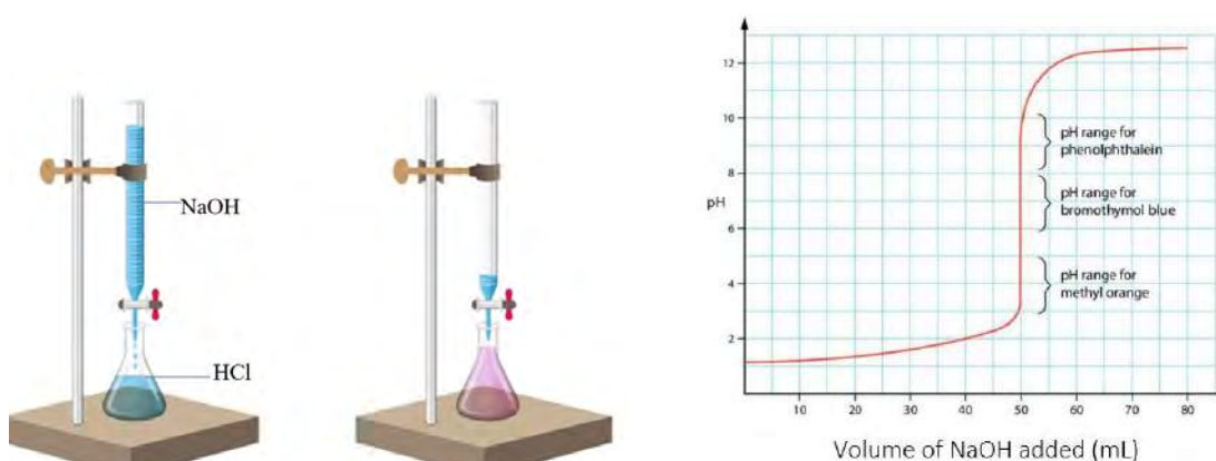
Figure: A graph of pH versus volume of alkali in the titration of strong acid and strong base
