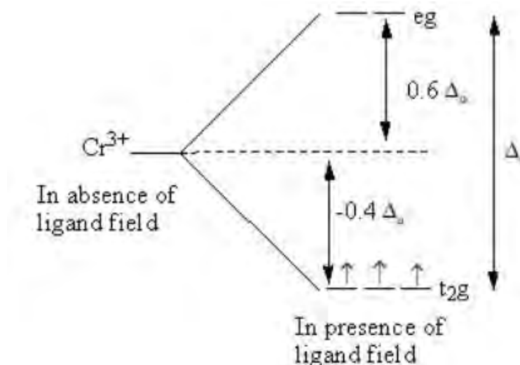
Octahedral field splitting of \text{Cr}^{3+}
