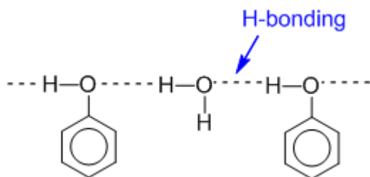
Fig: Hydrogen bonding between phenol and water.
