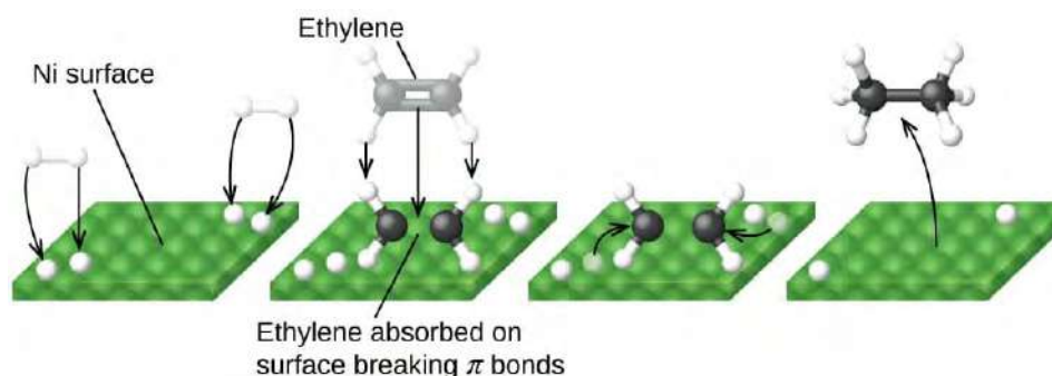
Figure: Hydrogenation of ethylene on the surface of nickel (heterogeneous catalyst)
