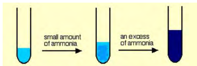
Fig: Formation of deep blue complex
