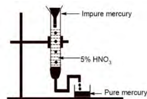
Fig: Purification of mercury
