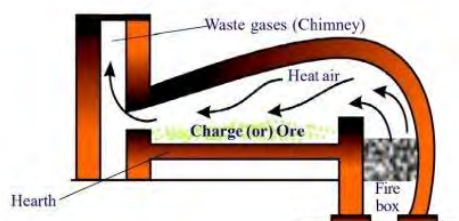
Fig: Reverberatory furnace for roasting
