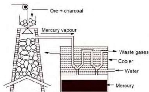
Fig: Shaft furnace for roasting & distillation
