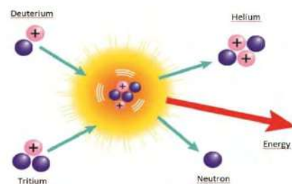
Fig: Nuclear reaction occurring in the sun
