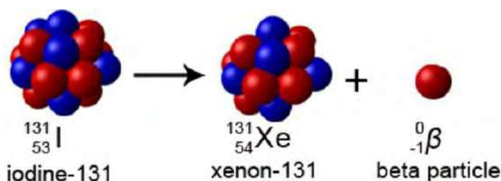
Fig: The beta particle emitted by iodine-131 has high energy and can kill cancerous cells.
