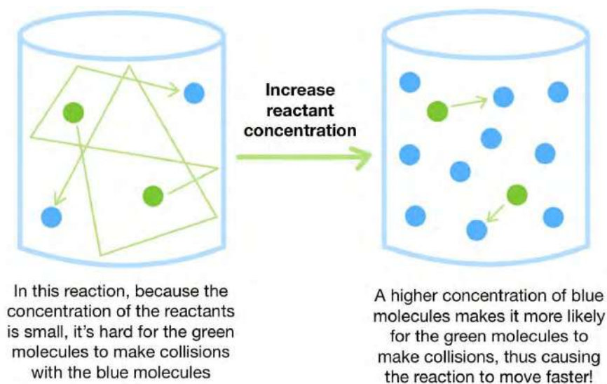
Figure: Effect of concentration on the rate of reaction
