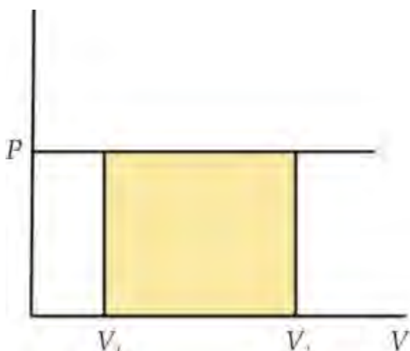
Figure : work done( W ) = P \times \text{change in volume}(\Delta V)
