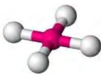
Fig: Square planar shape
