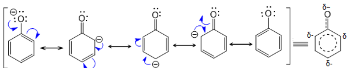
Fig: Resonating structures of phenoxide ion
