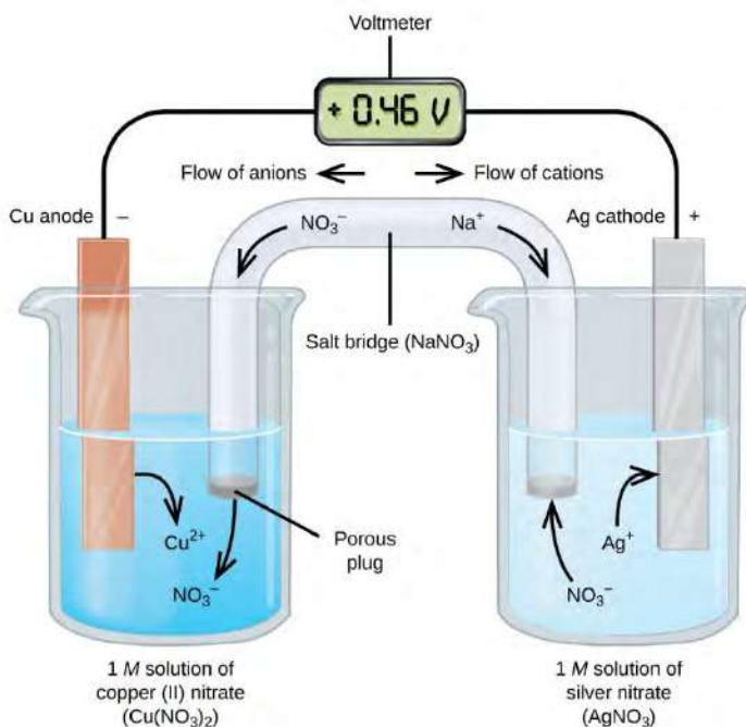
Fig 5.4.2: Representation of Cu-Ag cell
