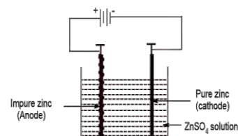
Fig: Electrolytic refining of zinc
