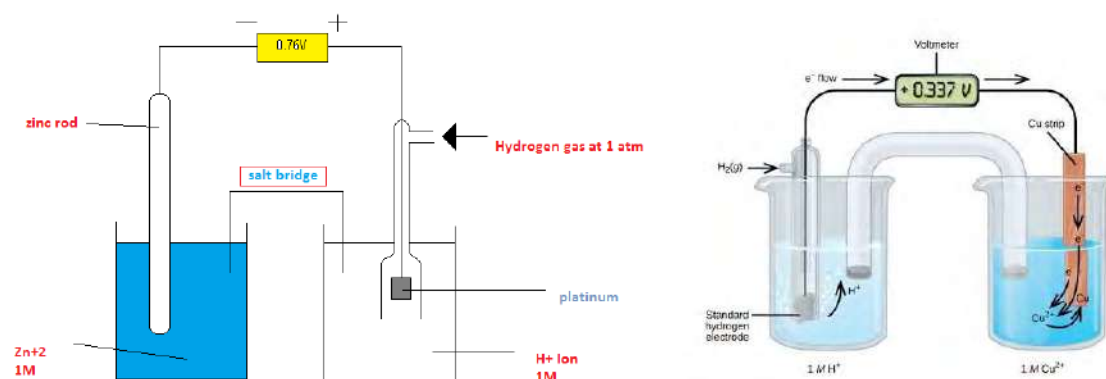
Fig 5.2.1: Measurement of electrode potential of zinc and copper
