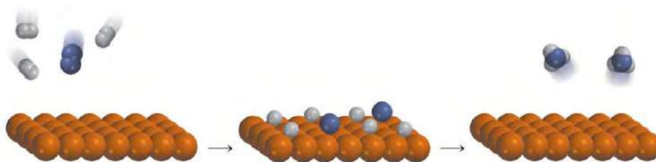
Figure: reaction of \text{H}_2 and \text{N}_2 in the surface of iron. Iron acts as a heterogeneous catalyst
