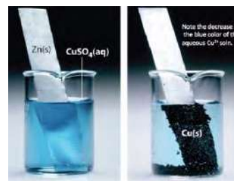
Fig: Zn displacing Cu from \text{CuSO}_4
