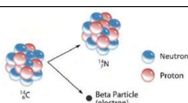
Fig: Decay of C-14
