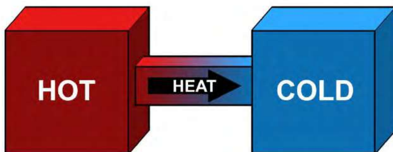
Fig : second law of thermodynamics explains the direction of heat flow
