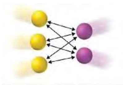
Fig : Collision among the molecules during the chemical reaction
