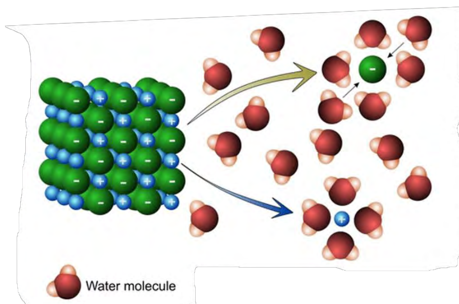
Figure: interaction of ions of salt with water.
