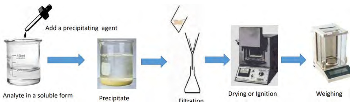
Figure 1.1. Diagrams illustrating the phenomena of gravimetric analysis
