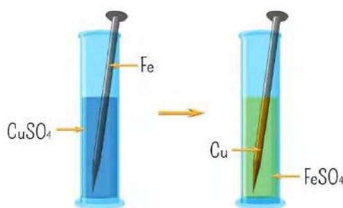
Fig 5.2.3.: Copper nail in \text{FeSO}_4 and iron nails in \text{CuSO}_4 solutions.
