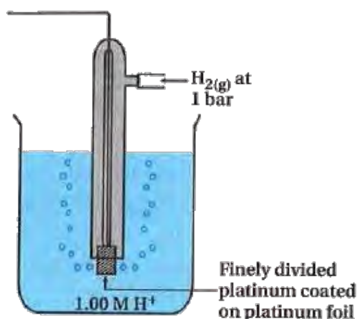
Fig 5.2: Standard hydrogen electrode
