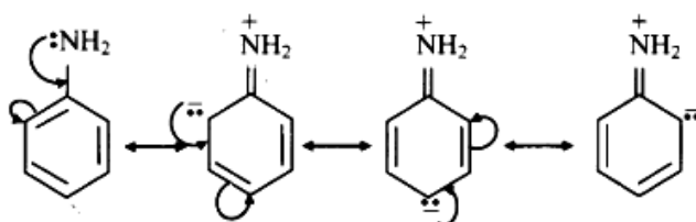
Resonance structures of aniline
