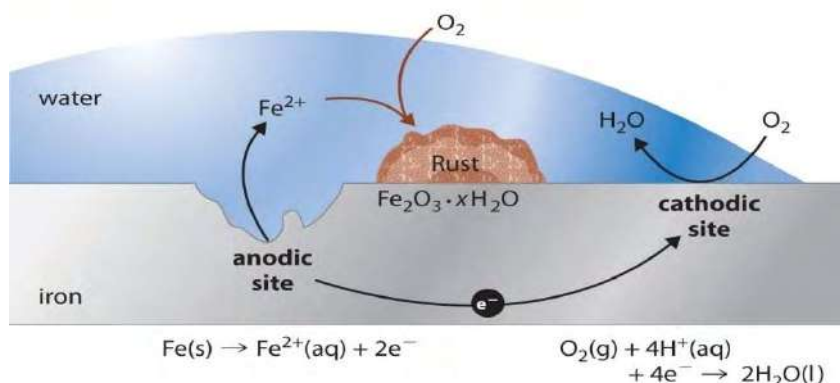
Fig: Electrochemical theory of rusting
