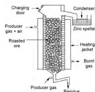
Fig: Vertical retort process for reduction of ZnO to Zn
